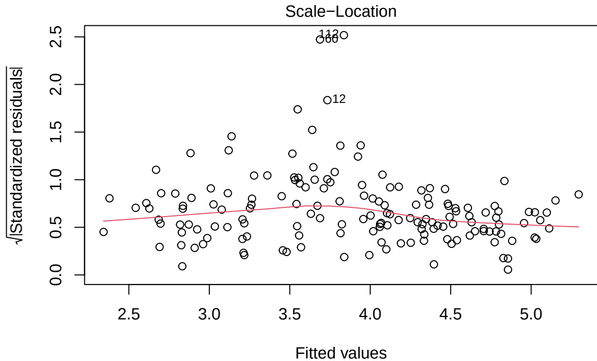
Figure 2.3: Scale location plot to test for homoscedasticity
